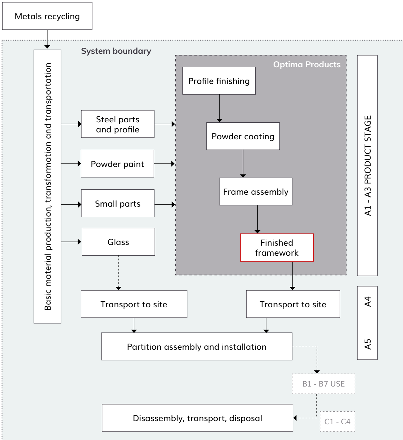
SYSTEM BOUNDARIES FOR TECHNISHIELD PARTITIONS LCA
