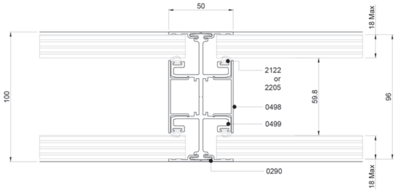
50mm mullion double solid panel
