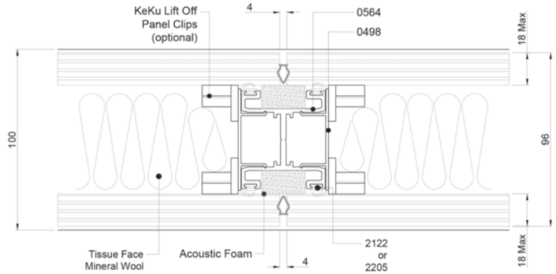
hidden mullion double solid panel
